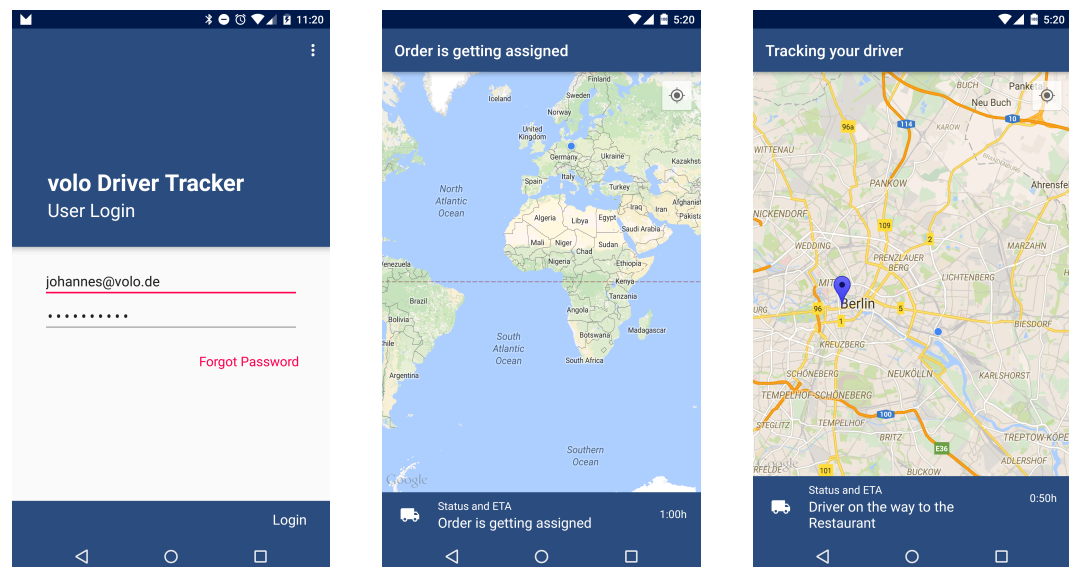
Figure 5.1: The consumer application. Login on the left. Driver has to be assigned in the middle. Delivery pick up has started on the right.
